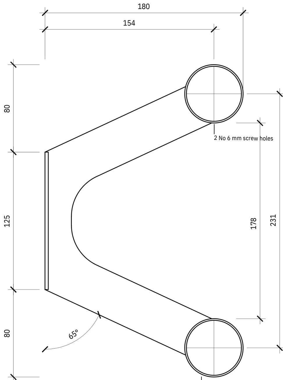
SIDE
