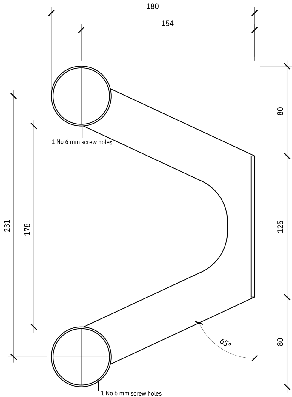
SIDE
